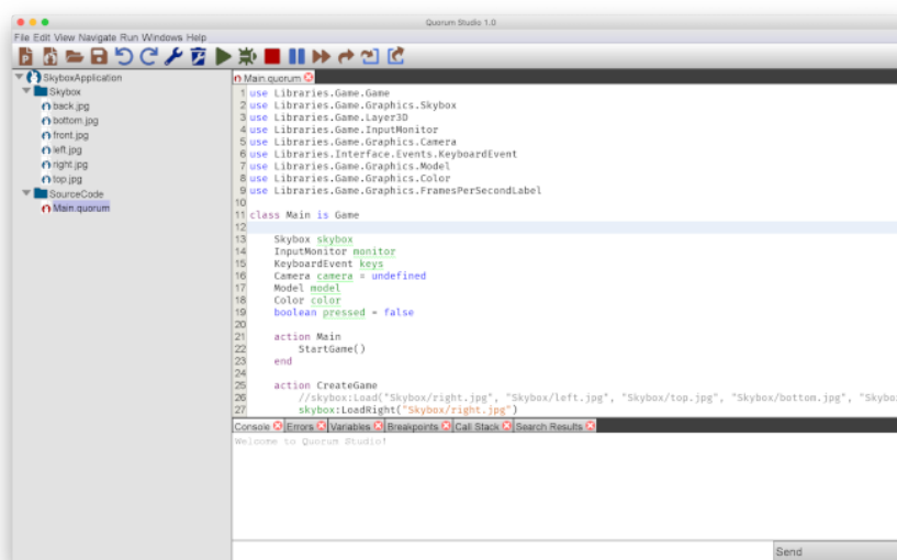
Obr. 1.3: Quorum
