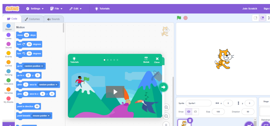
Obr. 1.6: Scratch
